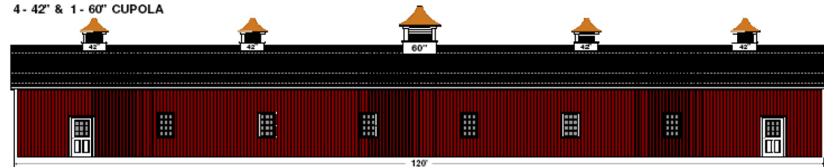
4 - 42" & 1 - 60" CUPOLA
